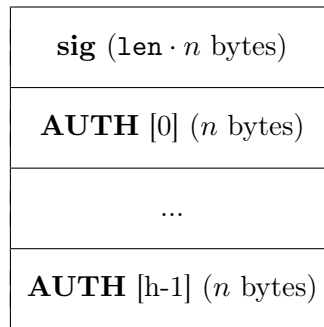
Figure 8: XMSS Signature
