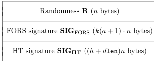
Figure 13: SPHINCS + signature
